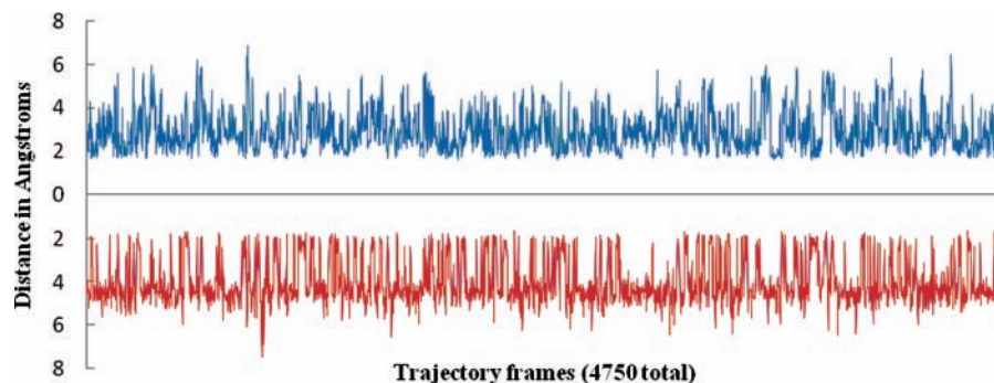
Figure 7. Top (blue plot): distance between the phosphate that connects DNA bases A5 and T6 and the closest amidine nitrogen of DB921. This is the same as D_1 in Figure 3. Each point is the distance for that particular frame. Bottom (red plot): distance between the phosphate that connects DNA bases T20 and C21 and the closest amidine nitrogen of the DB921 molecule. This is the same as D_2 in Figure 3. An inverted plot is used for D_2 . This enables the direct comparison of distances D_2 and D_1 at corresponding frames. Each point is the distance for that particular frame. There are a total of 2313 frames (i.e., 46.2 ns).
