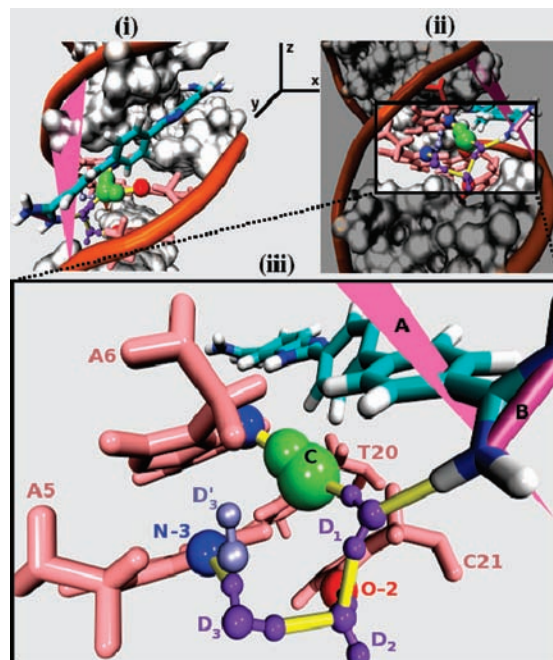
Figure 4. DB921–DNA complex in the perpendicular mode ( \perp -major). (i) DB921–DNA complex in a comparable orientation as Figures 2 and 3. (ii) With respect to the axis shown in (i), this orientation is obtained by rotating (i) by approximately 90^\circ counterclockwise about the z -axis and approximately 40^\circ clockwise about the x -axis. (iii) Magnified view of noncovalent interactions that are typical of the \perp -major mode of binding. The angle made by the line, labeled B, to the reference plane, labeled A, is close to 90^\circ ( \pm 20^\circ ), and thus the figures represent one of the perpendicular conformations ( \perp -major) observed in the MD simulation that is different from the X-ray crystal structure. The yellow cylindrical lines represent H bonds. (A) Plane of reference. (B) Line used to calculate the angle between the amidine groups to the reference plane. (C) Long residence time water, observed consistently in the simulation. The persistent H-bonding partners for this water are A6–N3 and T20–O2. (D1–D3) Water molecules that mediate transient H-bonding interactions involving A5–N3 and C21–O2 and stabilize the binding of DB921 to the minor groove (see text for description). (D3') Alternative orientation of the water molecule D 3 associated with A5–N3.
