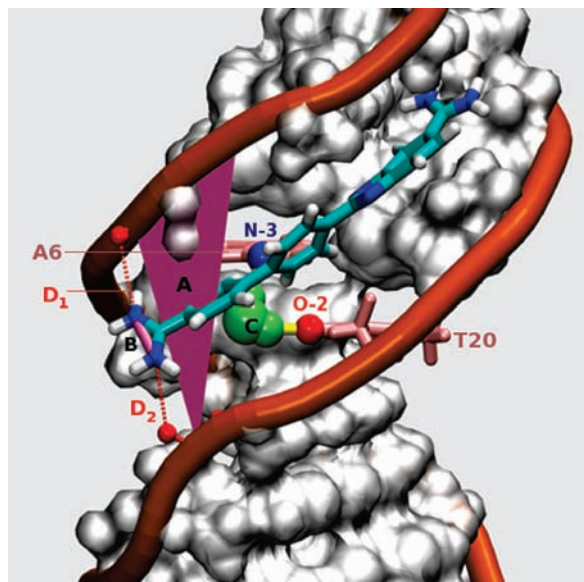
Figure 3. DB921–DNA complex in the parallel conformation (||). The angle from the line, labeled B (connecting N–N of the phenylamidine), to reference plane, labeled A, is close to 0^\circ ( \pm 20^\circ ), and thus the figure represents one of the parallel conformations (||) observed in the MD simulation. The yellow cylindrical lines represent H bonds. (A) Plane of reference constructed to computationally classify each frame (20 ps snapshot) into || or \perp modes of interaction. The plane is approximately parallel to the floor of the DNA minor groove (see text for details). (B) Line used to calculate the angle made by the amidine group to the reference plane (and hence, approximately to the floor of the groove). This angle is calculated for each snapshot of the MD and is used as an index to classify the frame into its respective binding mode. (C) Long residence time water observed consistently in the simulation. The persistent DNA H-bonding partners for this water are A6–N3 (labeled in blue) and T20–O2 (labeled in red). (D) Phosphate amidine electrostatic interactions are denoted by D 1 and D 2 (red dotted lines).
