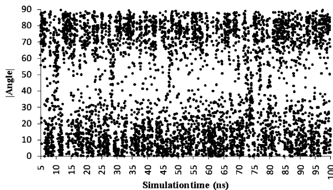
Figure 5. Scatter plot of angle made by the phenylamidine of DB921 (label B in Figures 3 and 4) and the reference plane (label A in Figures 3 and 4) across the length of the simulation. The y-axis is the absolute value of this angle, and the x-axis is the time during the simulation (5–100 ns). It is observed that there is a concentration of values around 0^\circ ( \pm 20^\circ ) and 90^\circ ( \pm 20^\circ ). The populations on the bottom and top of the plot are the groups of \parallel and \perp conformations, respectively.
