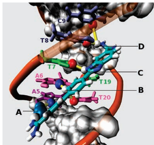
Figure 2. The DB921–d(CGCGAATTCGCG) 2 X-ray structure (PDB ID: 2B0K) with added protons. Yellow colored cylindrical lines represent hydrogen bonds formed between groups at the start and end points of the line. Hydrogen bonds are defined as interactions between acceptor and donor atoms that are less than 3.4 Å apart. (A) Water-mediated, hydrogen-bonding interaction between the phenylamidine of DB921 and A5-N3 (see numbering scheme in Figure 1, bottom) of the DNA minor groove. (B) Two short C–H···N/O-type interactions of –CH of the central phenyl of DB921 with A6-N3 and T20-O2. (C) Bifurcated H-bonded interactions of the inner benzimidazole nitrogen (–NH) with T7-O2 and T19-O2. (D) Bifurcated hydrogen bond between benzimidazole side amidine and T8-O2 and C9–O2.
